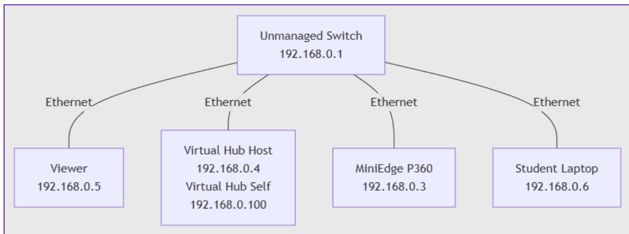
Figure 1: Portrait Mobile System setup. Static IPs already set on all devices besides Student Laptop
